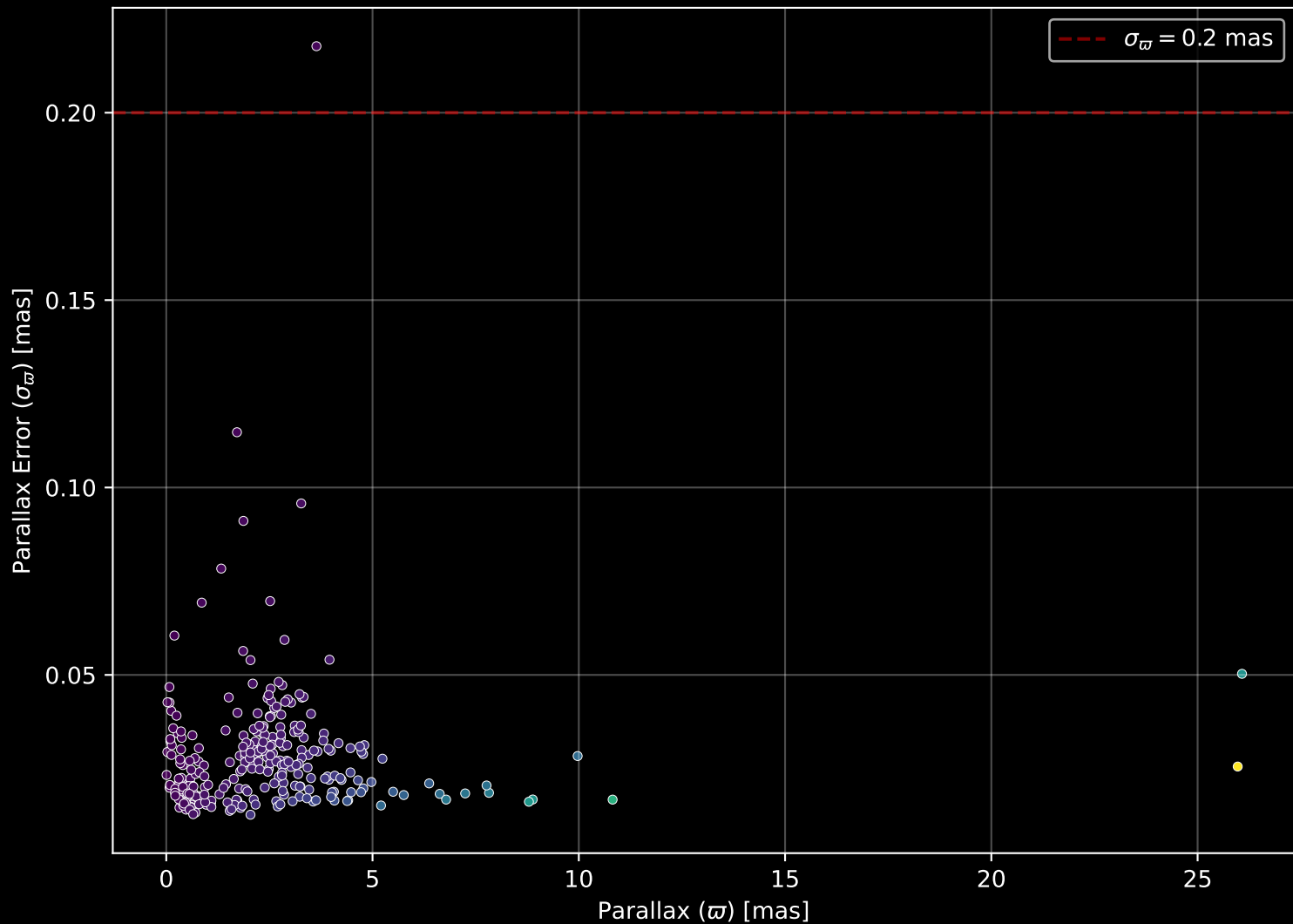
APOGEE DR17 Field: [SgrO3] Parallax Quality (n= 282)
