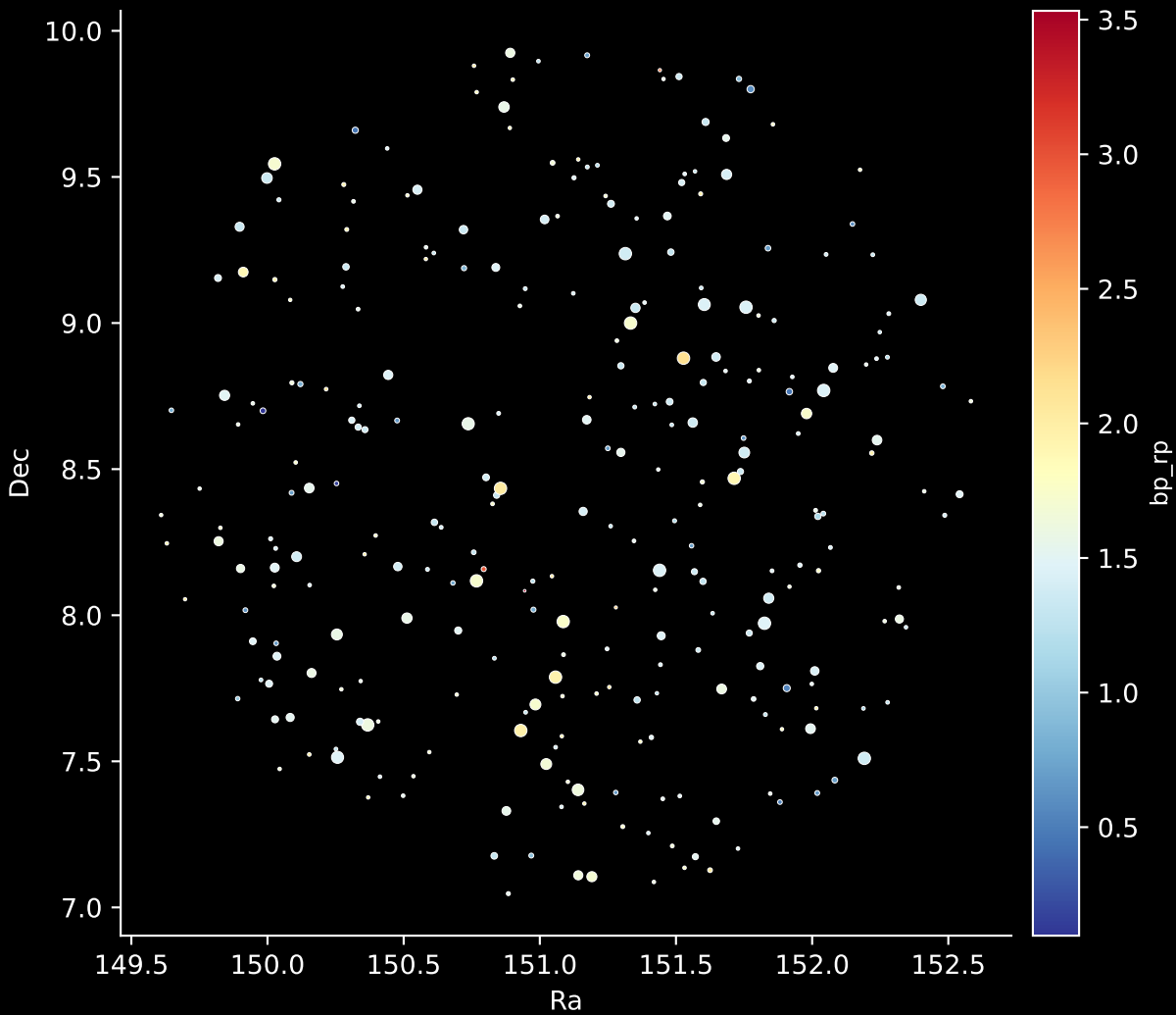
APOGEE DR17 Field: [SgrO3] Stars: 282
