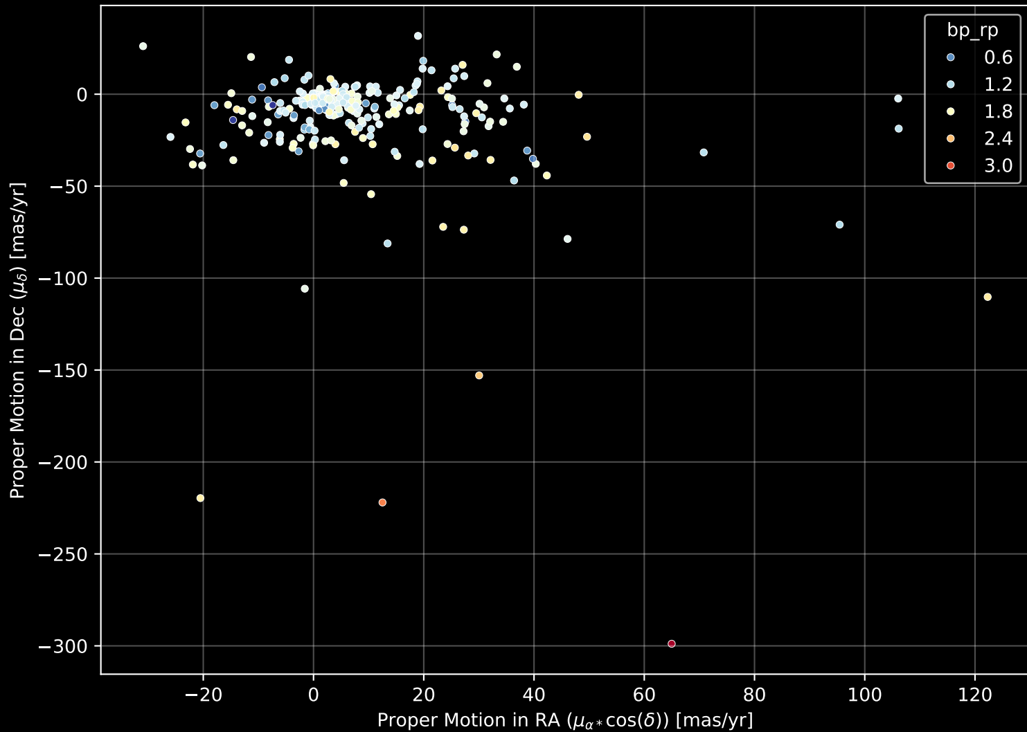
APOGEE DR17 Field: [SgrO3] Proper Motion Diagram (n= 282)
