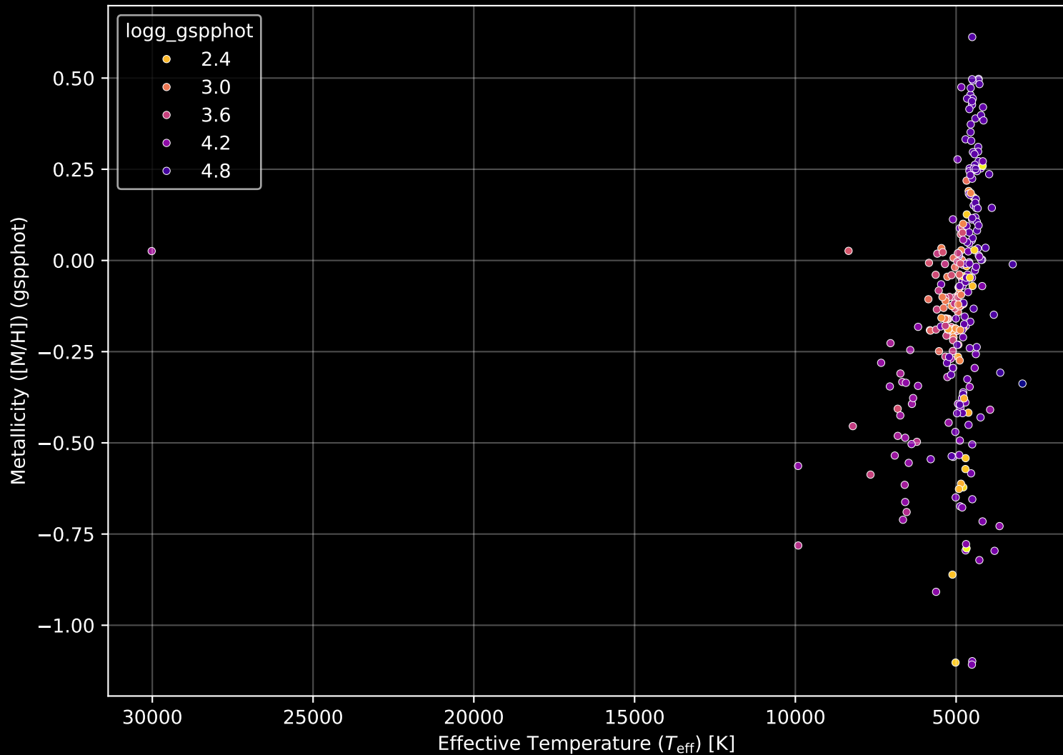
APOGEE DR17 Field: [SgrO3] Stellar Population Parameters (n= 282)
