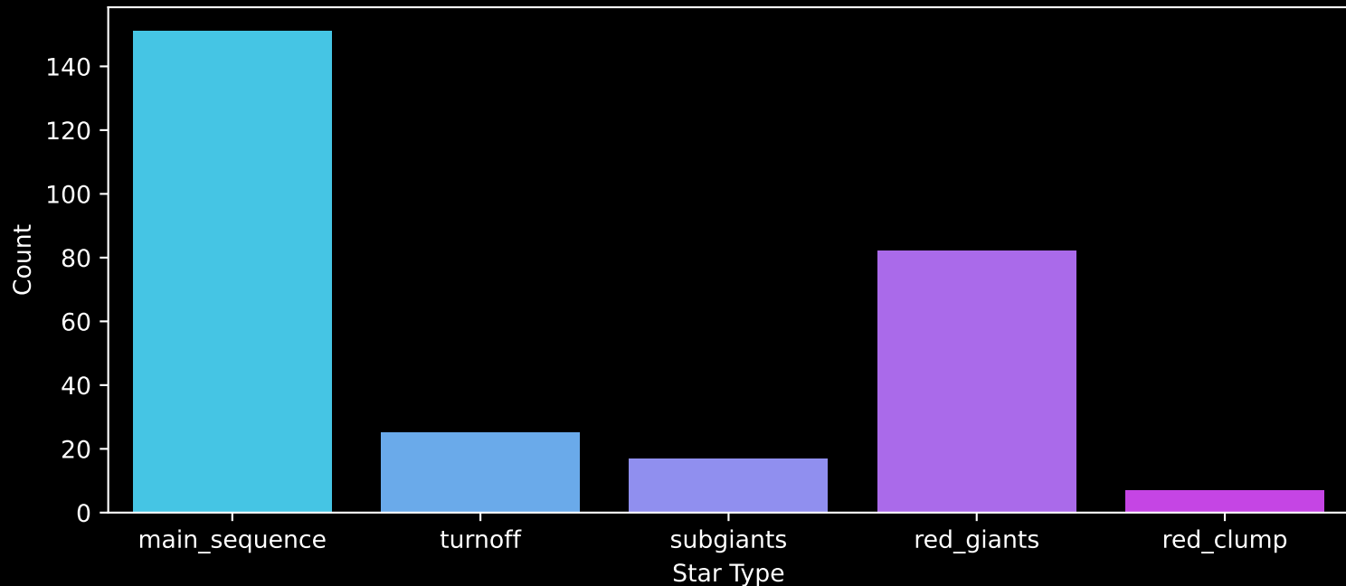
APOGEE DR17 Field: [SgrO3] Count plot of Star Type
