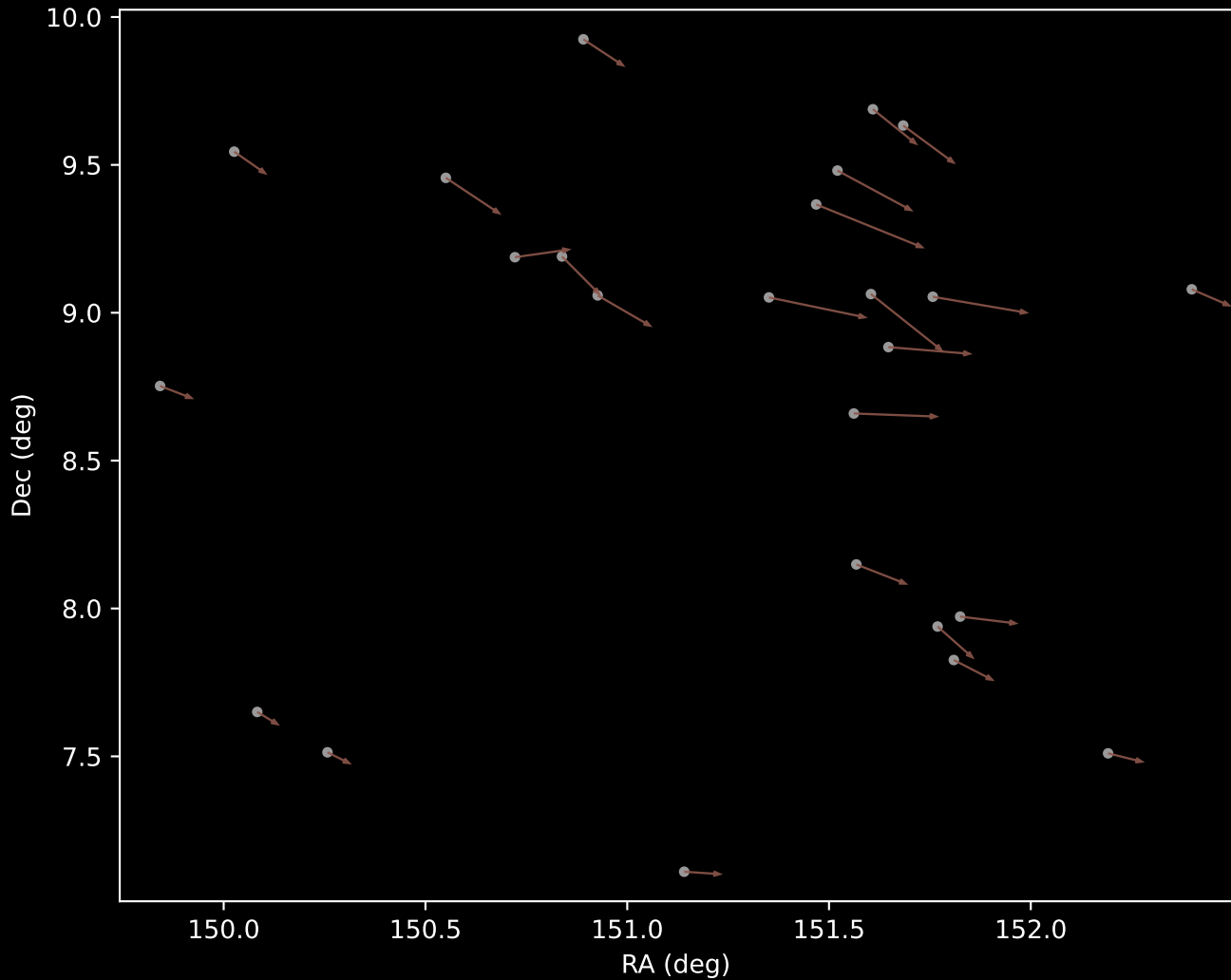
APOGEE DR17 Cluster 10 Proper Motion Vectors (n=25)
