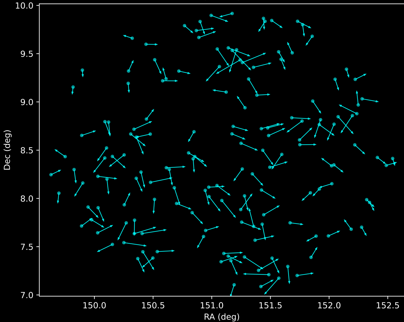
APOGEE DR17 Noise Stream Proper Motion Vectors (n=157)
