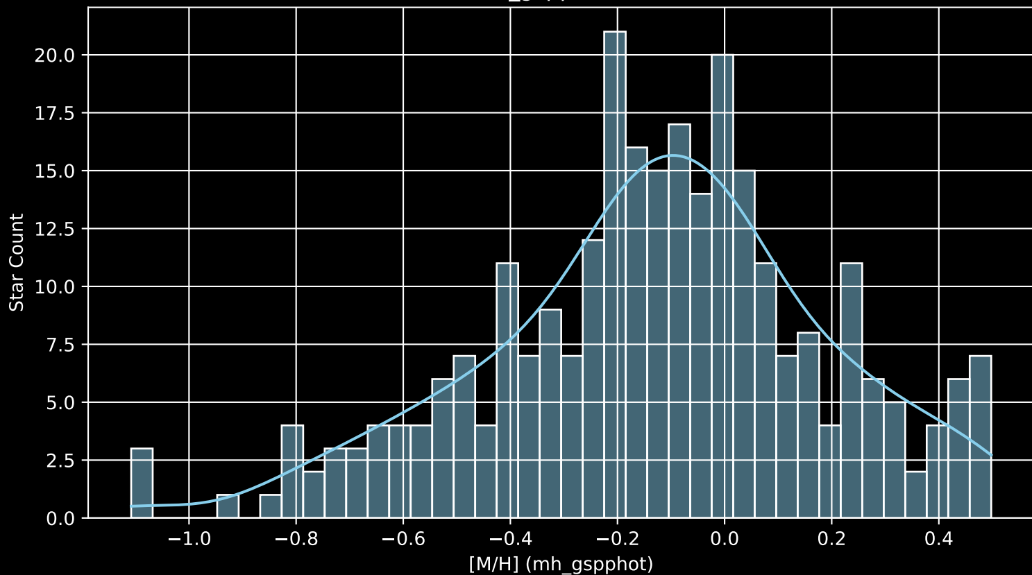
APOGEE DR17 Field: [SgrO3 [M/H] (mh_gspphot) (n= 281)
