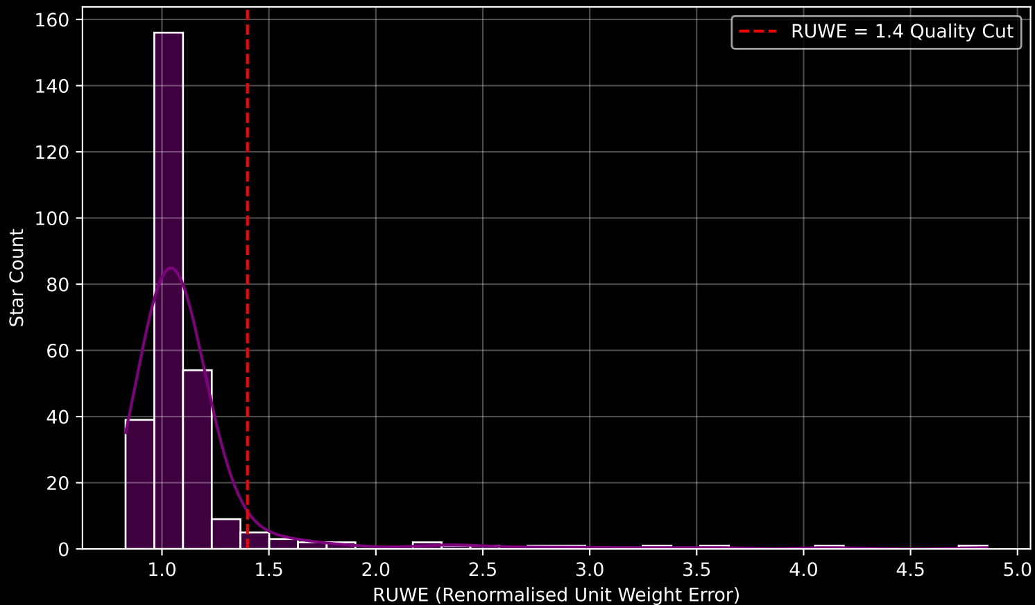
GAPOGEE DR17 Field [SgrO3] RUWE Distribution (n= 280)
